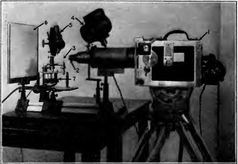
FIG. 1. Taking motion pictures of a carbon particle on the point of a needle. (1) Camera, (2) objective, (3) carbon particle on needle, (4) (5) light-sources, (6) back drop, (7) rotating device.
